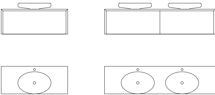
B-1485 120 x 50 x 45H [1 CAJÓN / 1 DRAWER]
