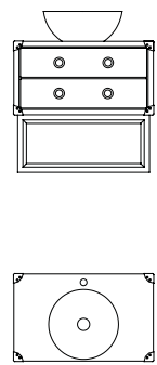
B-1500 80 x 50 x 75H [2 CAJONES / 2 DRAWERS]
